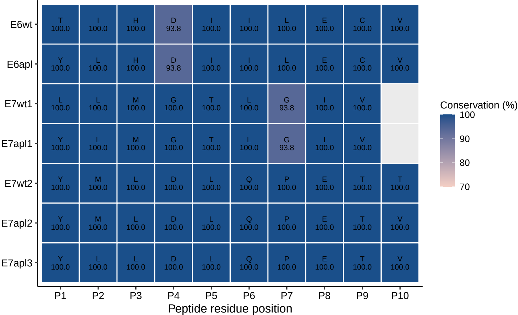
Epitope-level conservation of HPV16 E6/E7 WT epitopes and APL candidates
